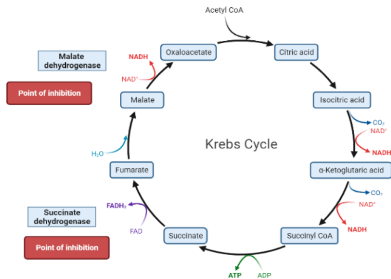
Figure 6. Krebs cycle.
