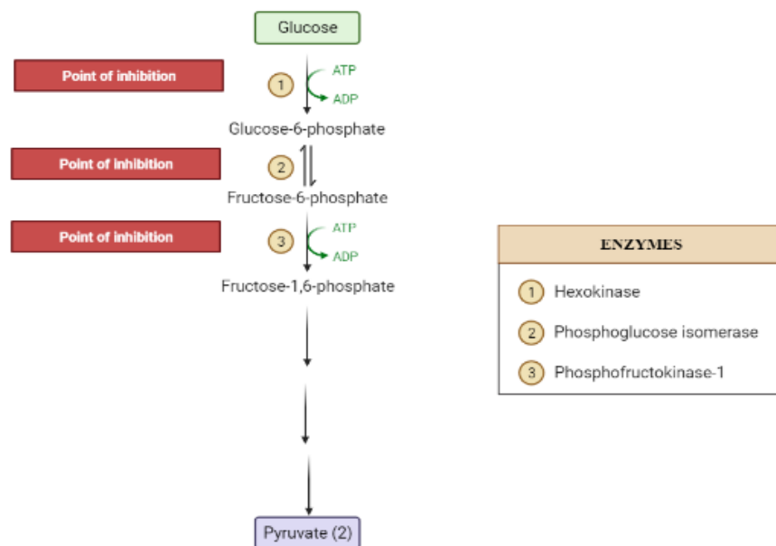
Figure 5. Glycolysis.
